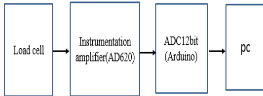
Figure (3). Schematic of basic system block diagram..
