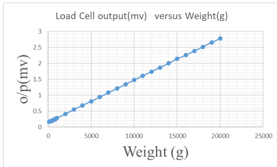
Figure (4) Load cell linearity.
